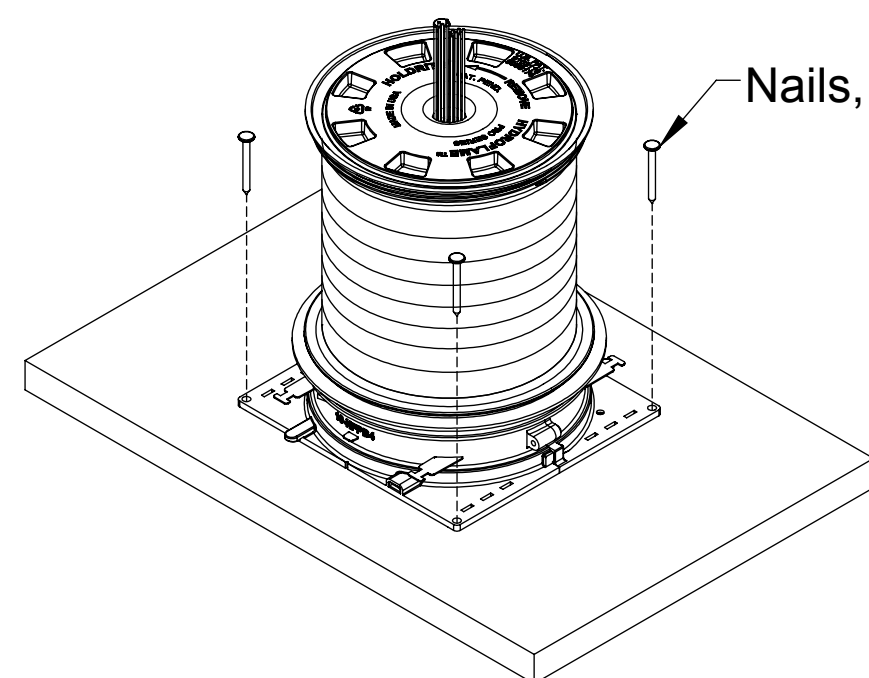
NAIL TO FORM DECK. (Fig. 4)
