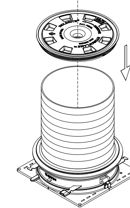
RE-INSTALL CAP & INSERT LOCATOR WHISKERS. (Fig. 3)
