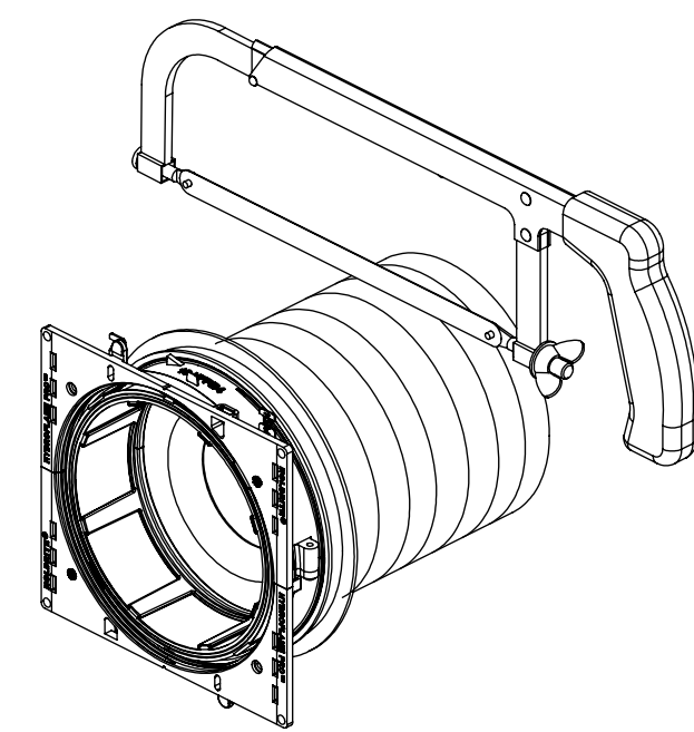
CUT SLEEVE, IF DESIRED HEIGHT IS UNDER 7-3/4". (CAN BE CUT AS SHORT AS 2-1/2") (Fig. 2)
