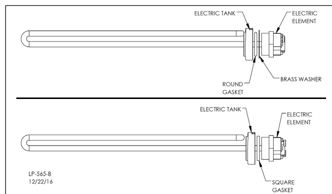
Figure 7 - Heating Element Detail
