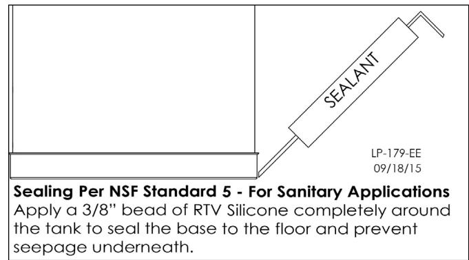
Figure 5 - Sealing the Water Heater for Sanitary Applications
