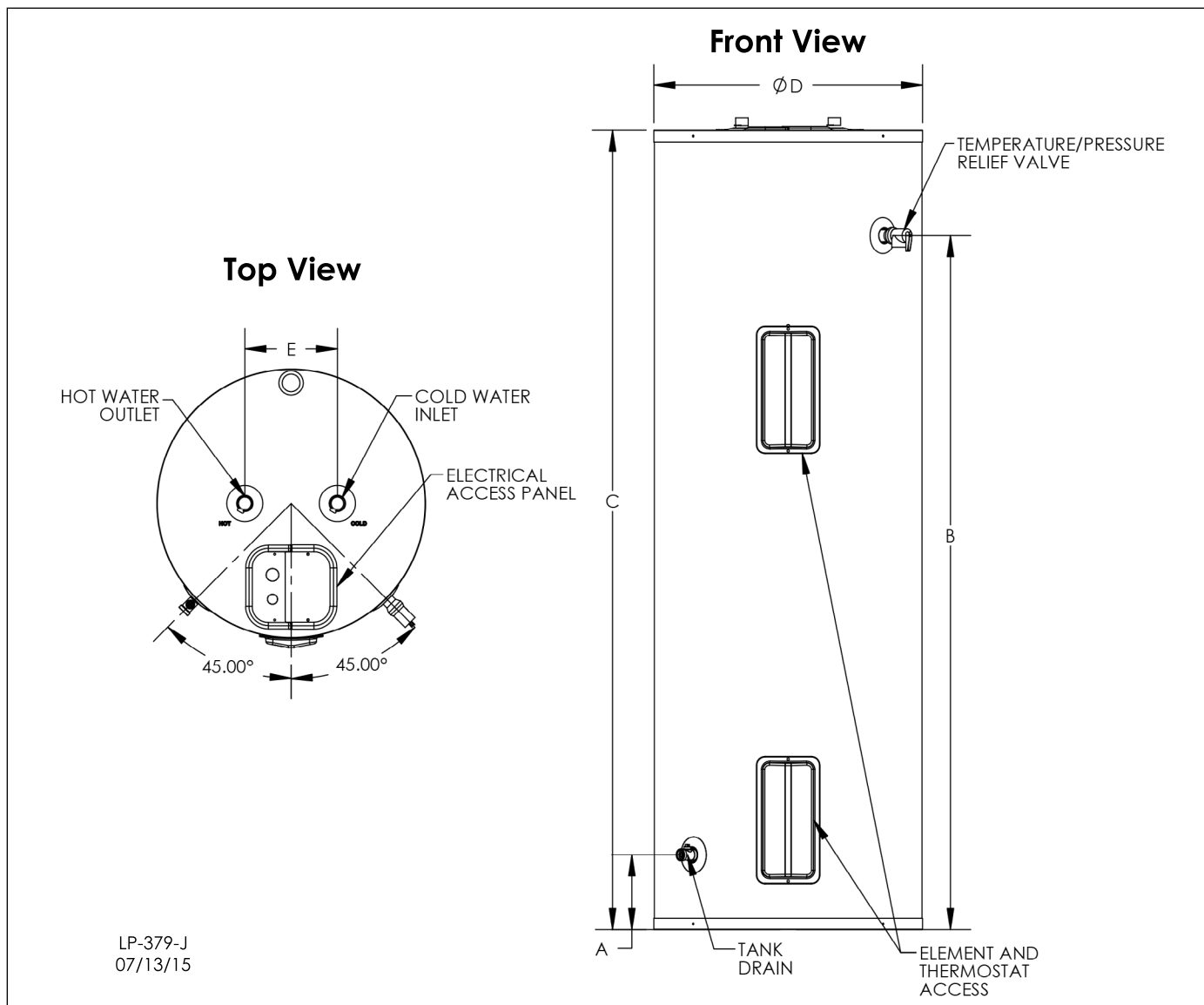
Figure 2 - Dimensional Drawing - Non-Simultaneous Operation
