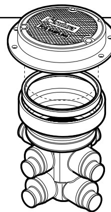
Endura Sampling Well with Cast Iron Cover
