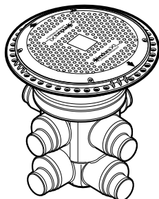
Endura Sampling Well with Traffic S-Rated Cover
