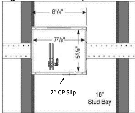
Right Hand Drain Option
