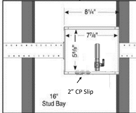
Left Hand Drain Option
