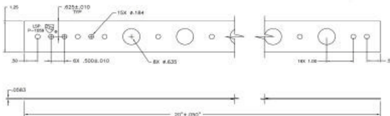
Part shown= P-1059
