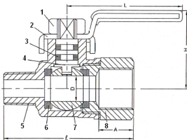
With Lever Handle
