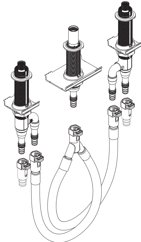
TWO-HANDLE ROMAN TUB VALVE WITH DURA-GRIP™ MOUNTING SYSTEM MODEL 4794
