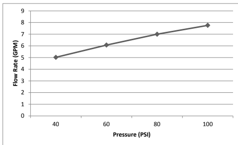
P-2307B Flow Rate (GPM) Vs Pressure (PSI) For Tub Port*
