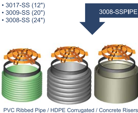
PVC Ribbed Pipe / HDPE Corrugated / Concrete Risers
