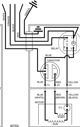
WIRING DIAGRAM FOR MODEL RE810 3/13 thru Current
