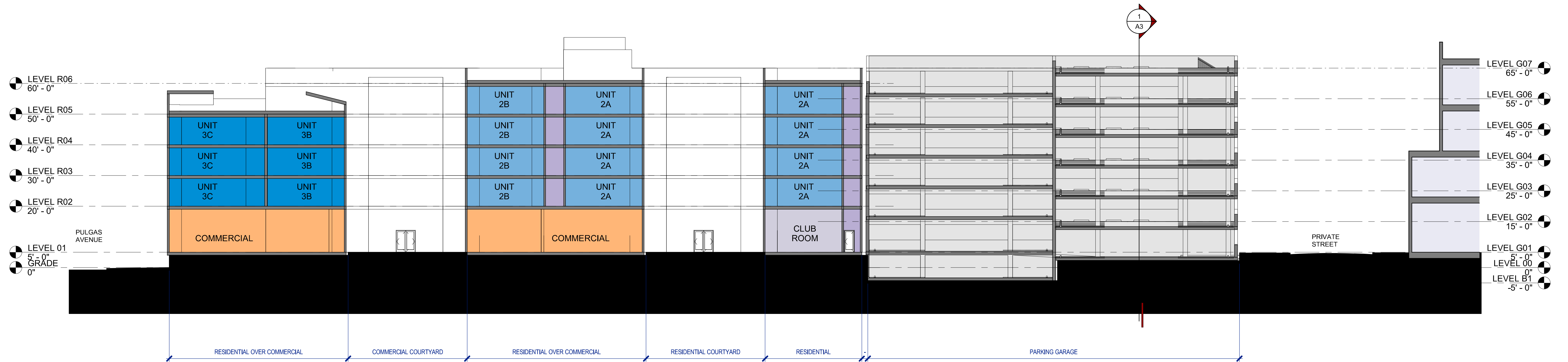
BUILDING SECTION THROUGH RESIDENTIAL & GARAGE LOOKING NORTH 2 1/16" = 1'-0"
