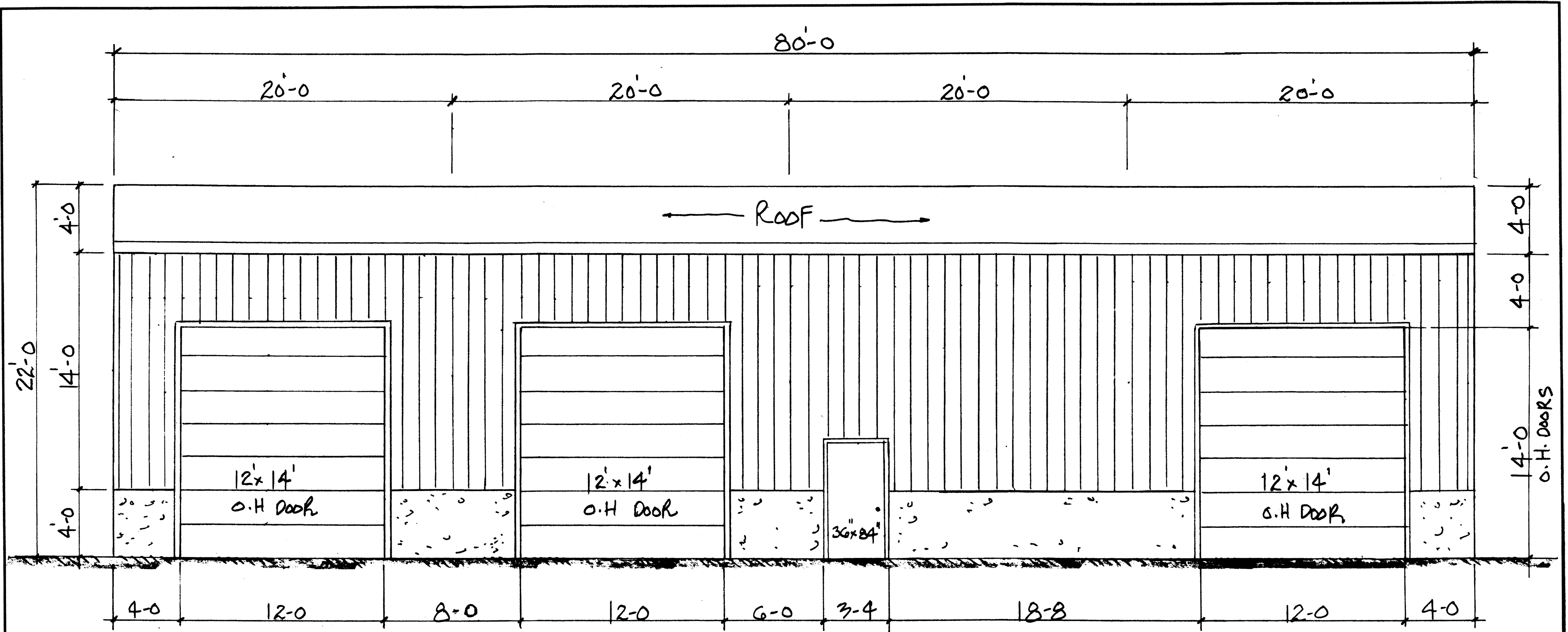
FRONT ELEVATION
