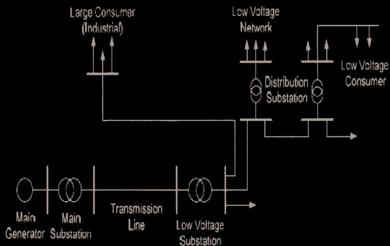
Fig. 1. Distribution Network.
