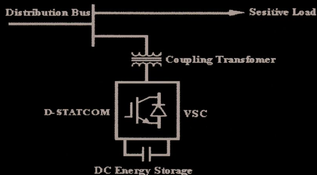
Fig. 2. Basic Configuration of D-STATCOM.
