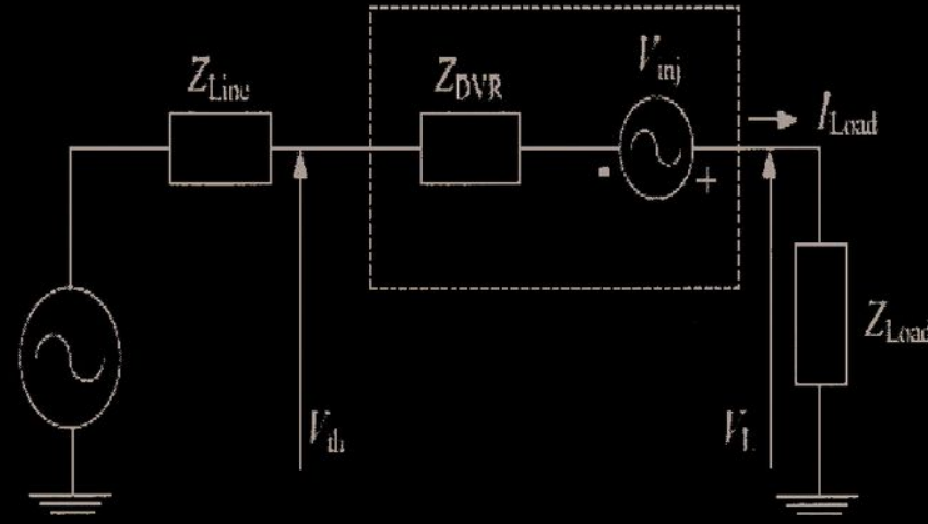
Fig. 5. Equivalent circuit of DVR.
