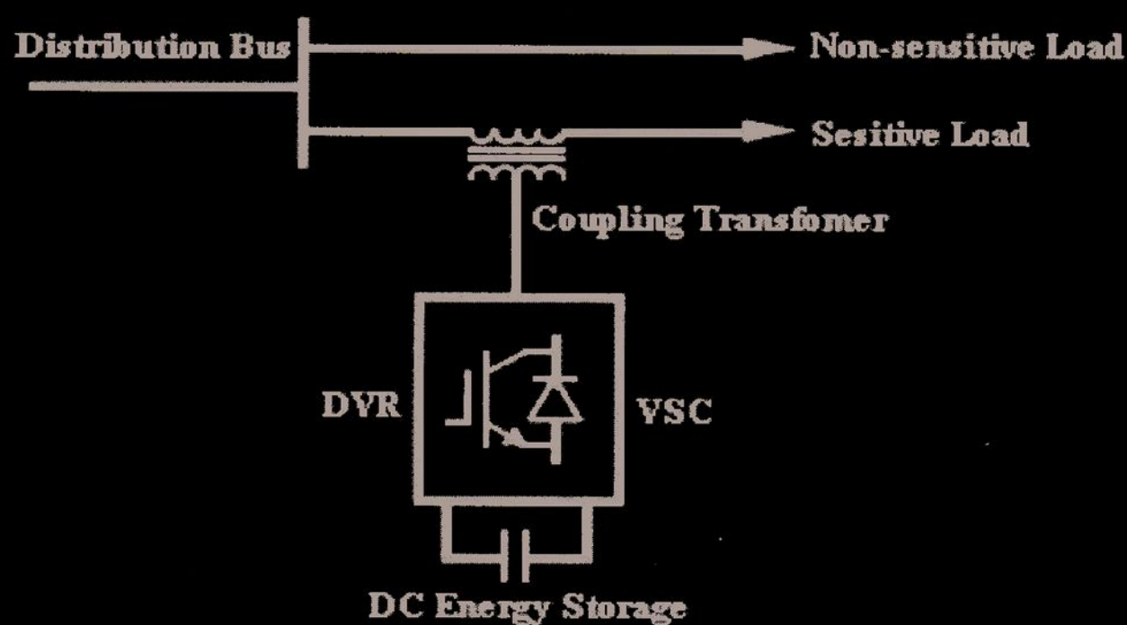
Fig. 4. Basic Configuration of the DVR.
