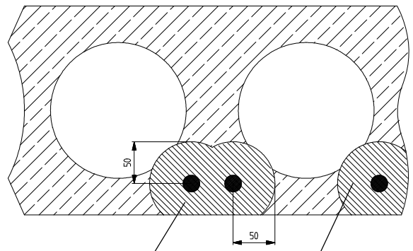
Area where no anchoring is allowed
