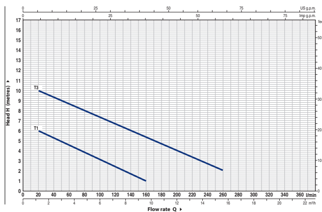
Performance curves RIVER Drain T1 GE and T3 GE
