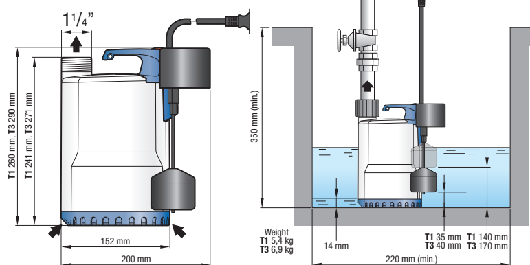
Dimensions RIVER Drain T1 GE and T3 GE
