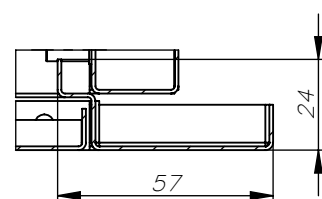
DETAIL P SCALE 1 : 2
