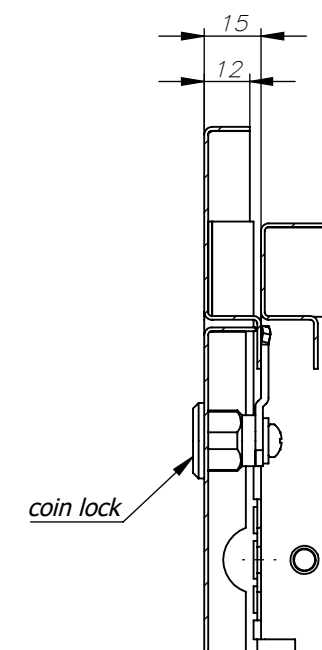
DETAIL N SCALE 1 : 2
