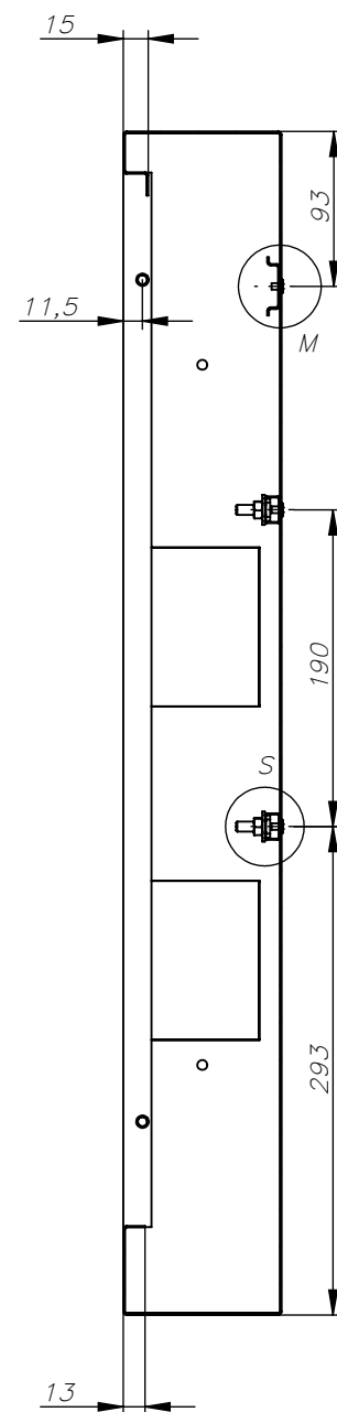
CROSS-SECTION B-B
