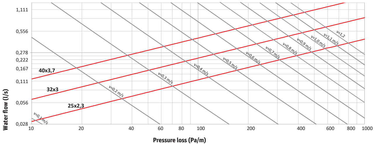
Pressure loss diagram PE-RT S3 at 40°C
