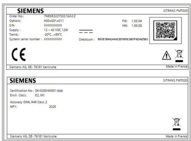
Transmitter label
