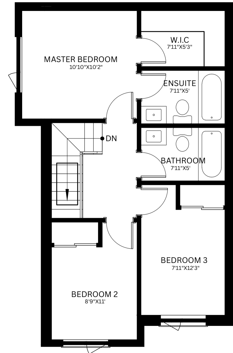
SECOND FLOOR
