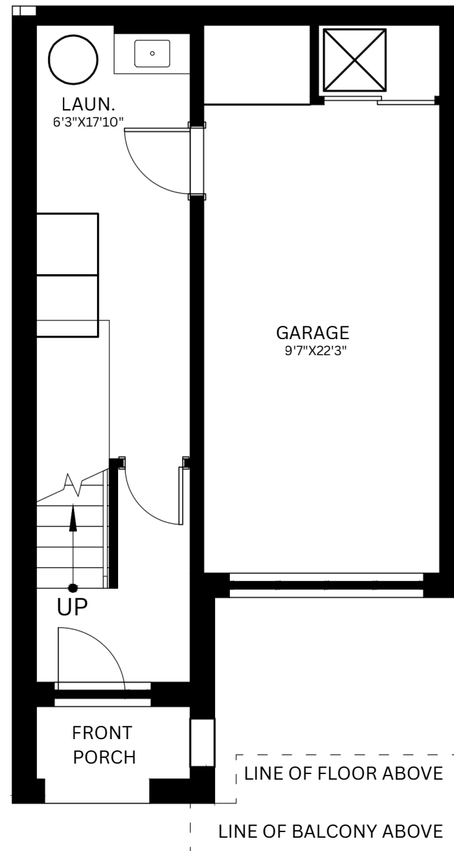
GROUND FLOOR
