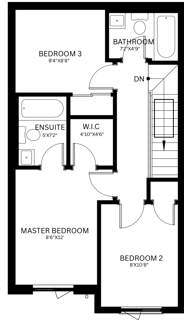
SECOND FLOOR
