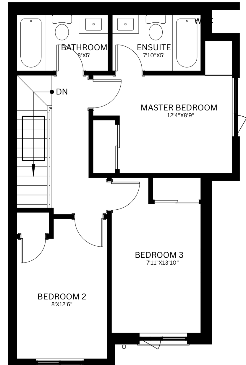
SECOND FLOOR
