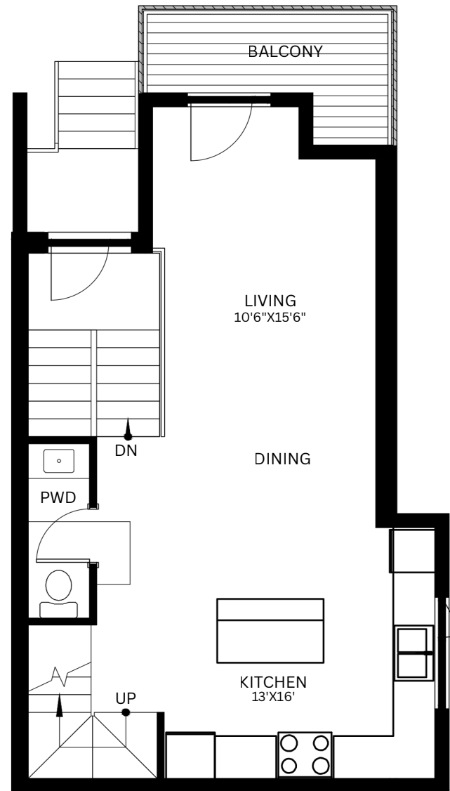
MAIN FLOOR
