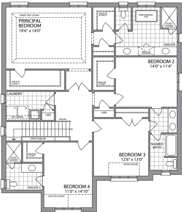
SECOND FLOOR ELEV B
