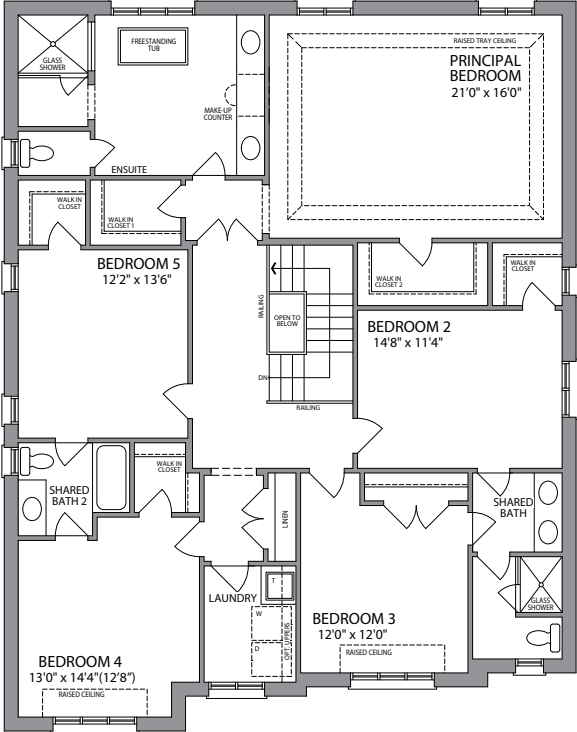
SECOND FLOOR ELEV B
