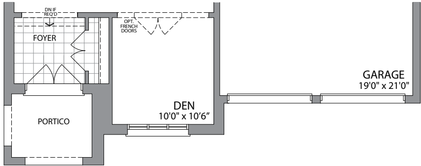
GROUND FLOOR ELEV B
