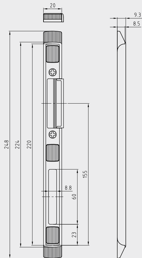
134/HS/20/11/x/DS
