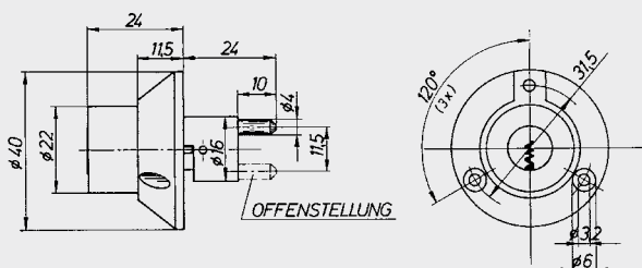
SYST/MZ_KP/1336/D22
