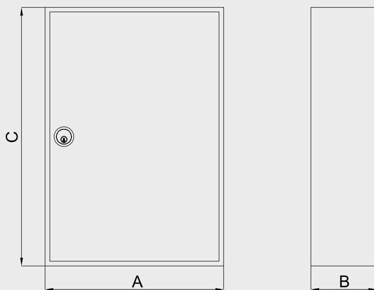
Schlüsselkasten SK
