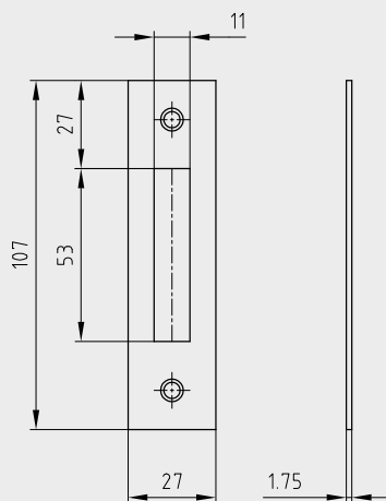
SB/SH.2/DS
