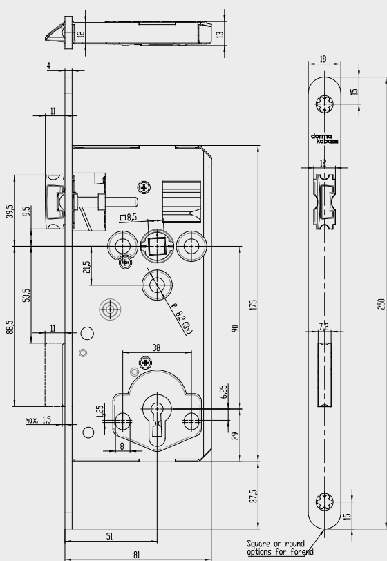
127/KB/FF/R/50/90/8,5/DS/250.18.4
