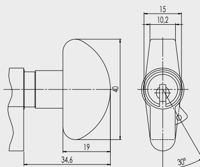
DKZ_AK583 Hebel Knopf
