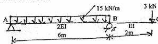
Figure: Load on beam
