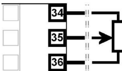
Figure 17. Input 2 - Potentiometer Connections
