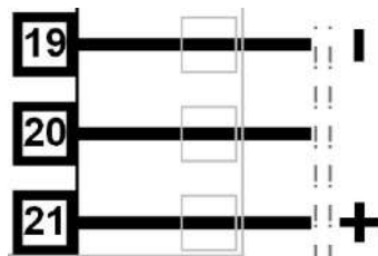
Figure 23. Plug-in Module Slot 1 – Single SSR Driver Module
