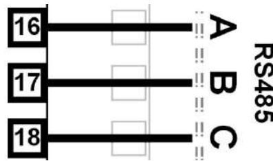
Figure 39. Plug-in Module Slot A – RS485 Serial Communications Module
