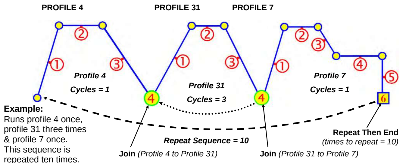
Figure 53. Profile Cycles & Repeats
