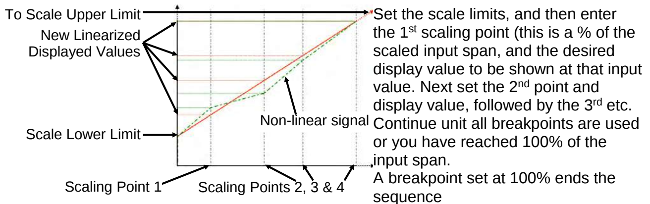
Figure 46. Multi-point Scaling
