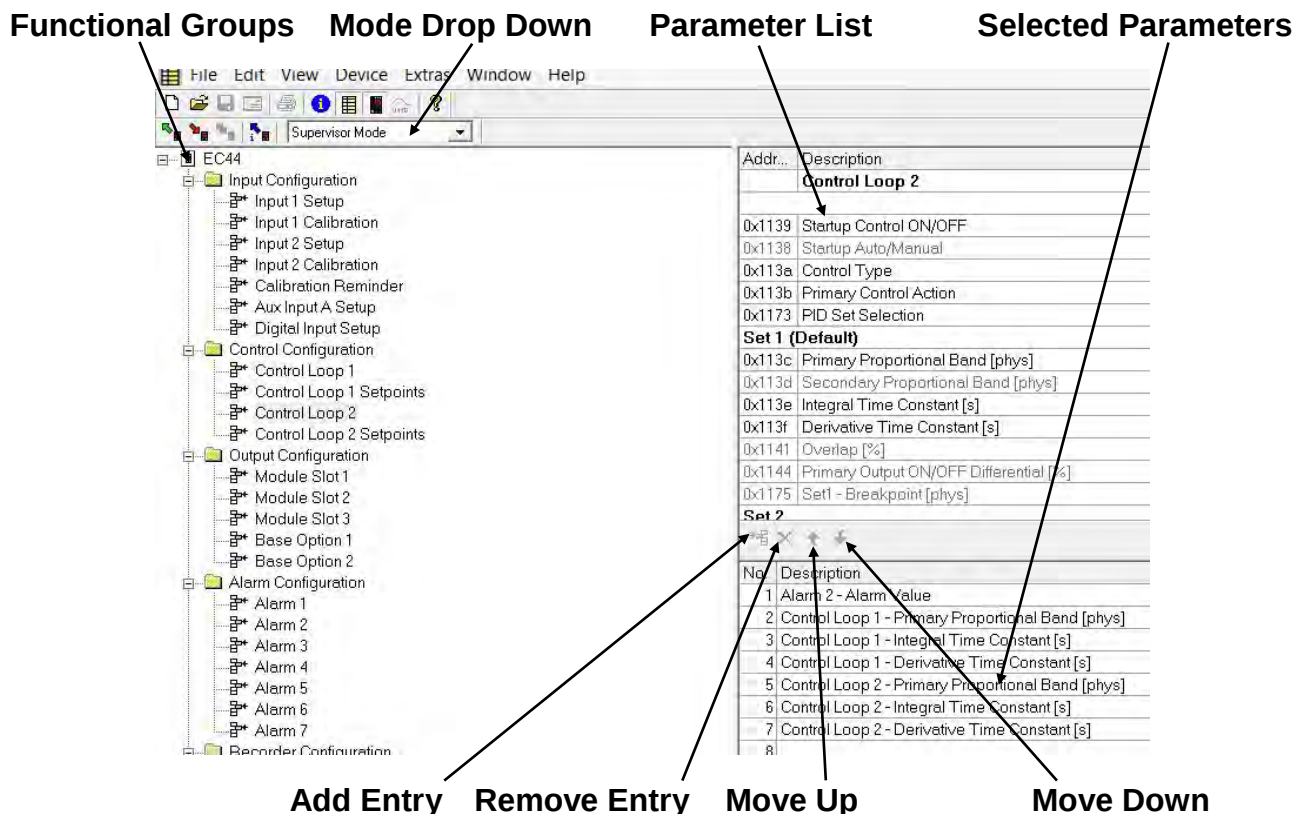
Figure 67. Supervisor/Enhanced Operation Mode Configuration
