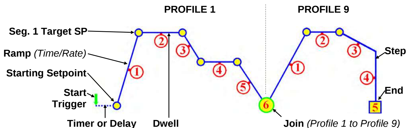
Figure 48. Profile Starting and Standard Segment Types
