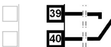
Figure 20. Relay Output 5 Connections
