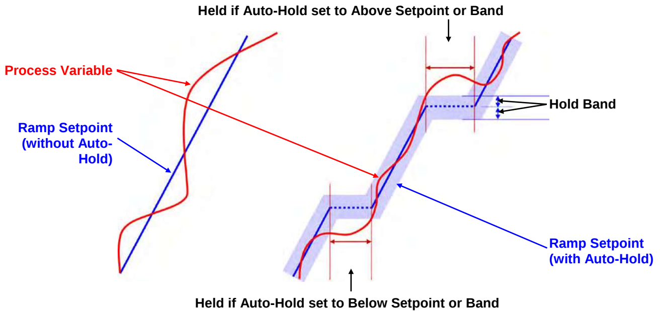
Figure 52. Auto-Hold On A Ramp Segment
