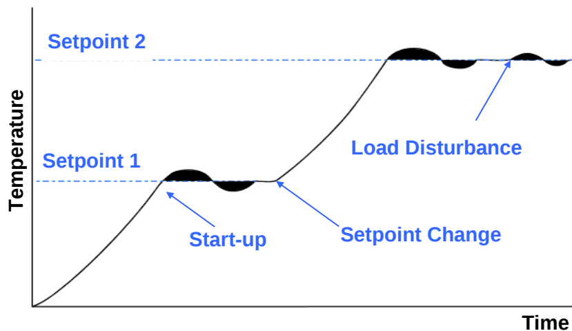
Figure 58. Self-Tune Operation
