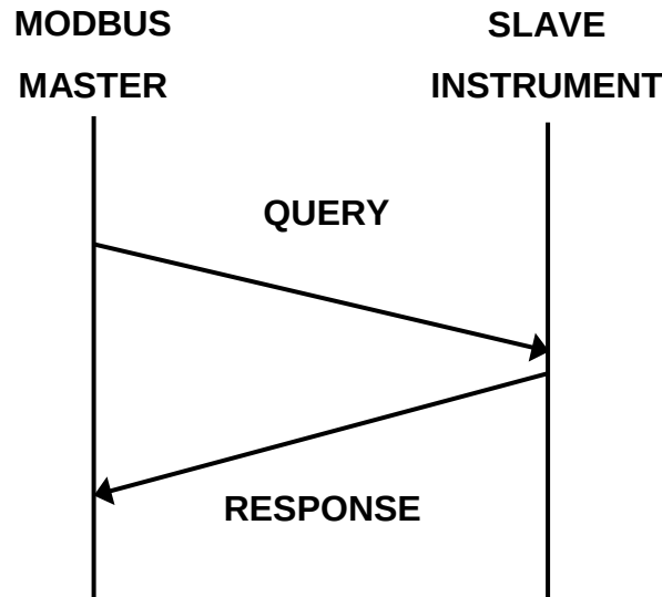
Figure 61. Modbus Link Layer
