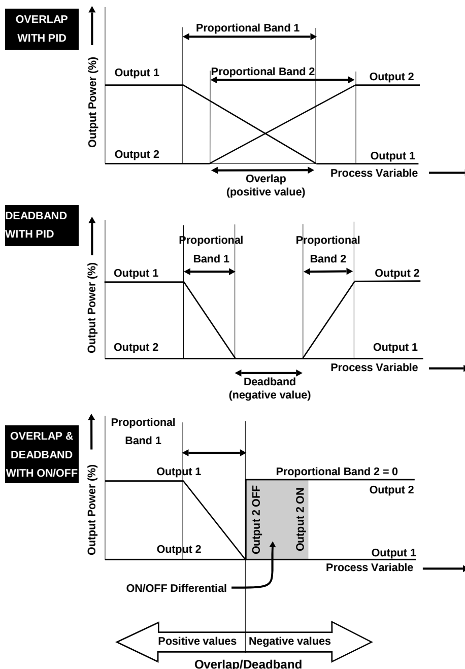
Figure 63. Overlap/Deadband
