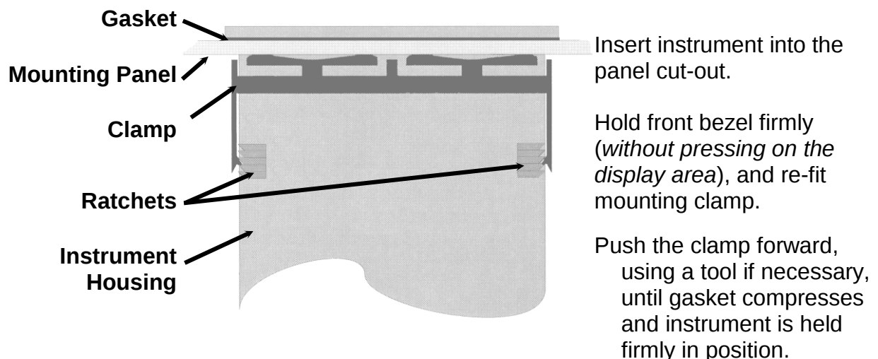
Figure 2. Panel-Mounting the instrument
