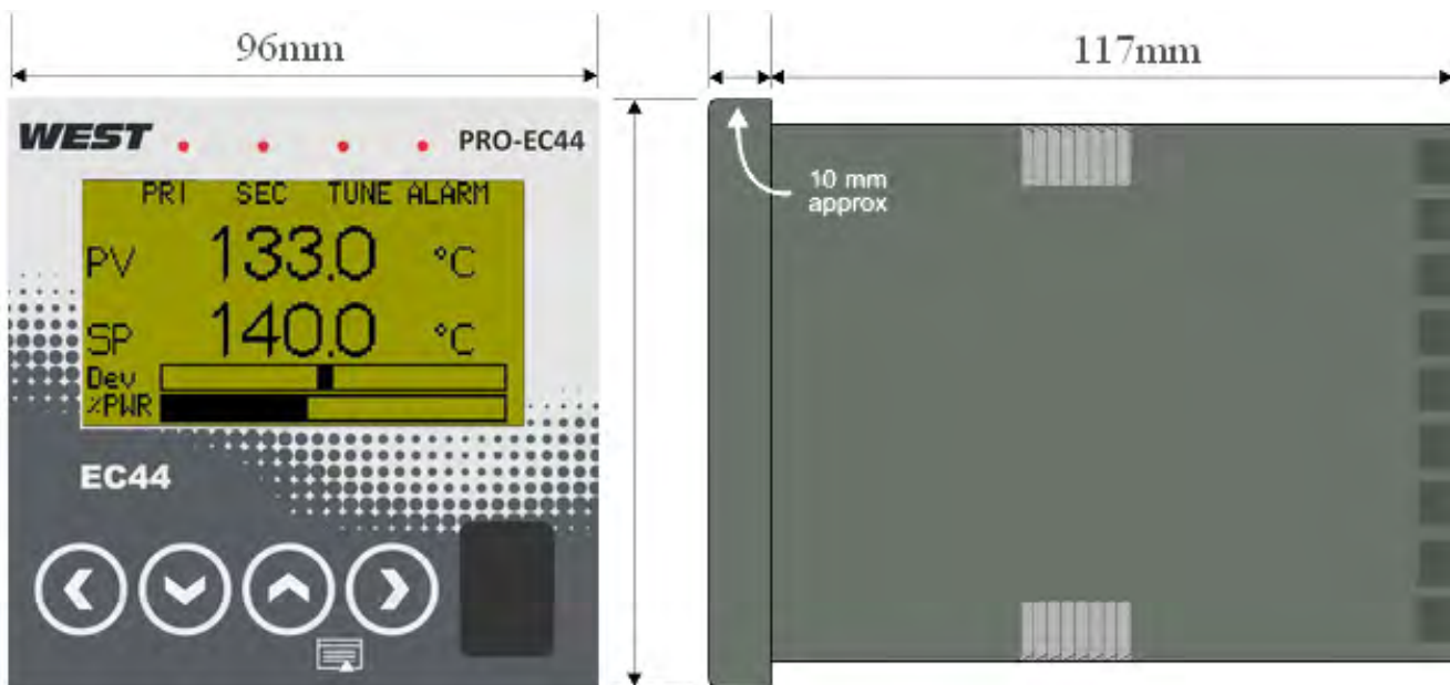
Figure 1. Main dimensions
