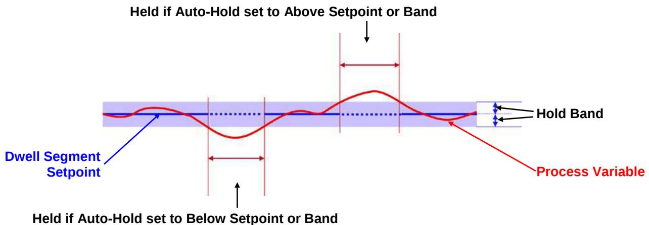
Figure 51. Auto-Hold on a Dwell Segment
