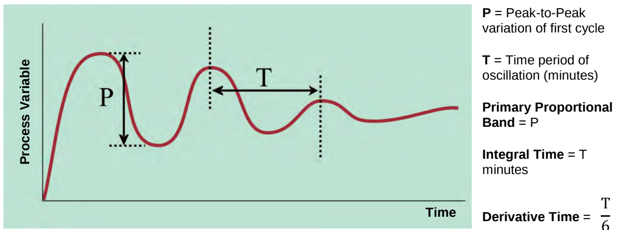
Figure 59. Manually Tuning - PID with Primary Output
