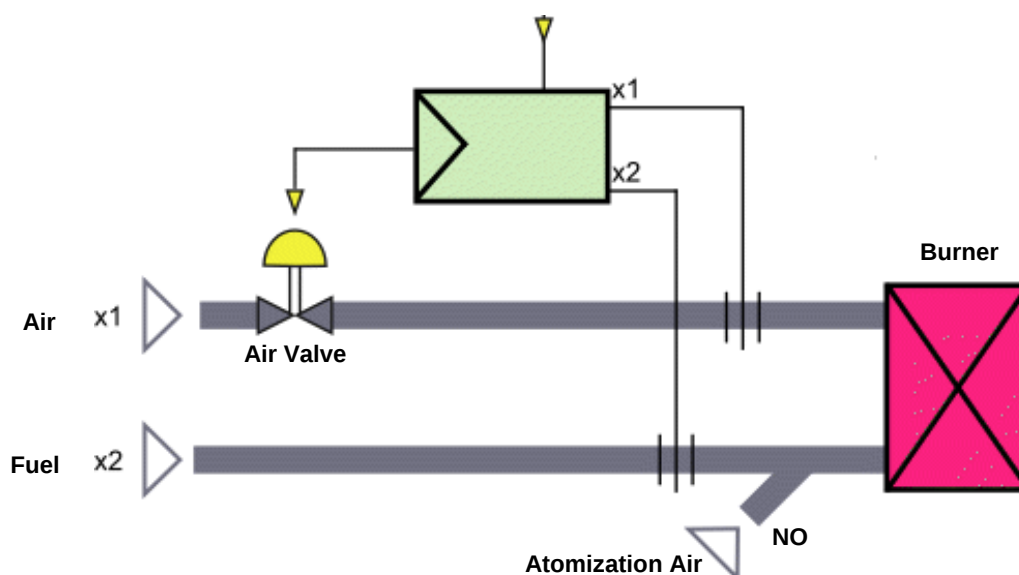
Figure 47. Ratio Control Example
