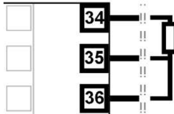
Figure 15. Input 2 - RTD Connections
