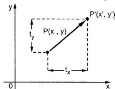
Figure 1: 2D Translation
