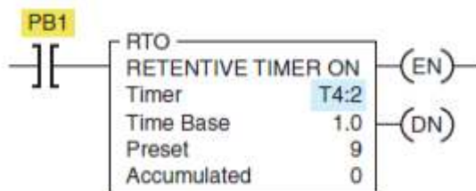
Fig 6.3: Retentive Timer instruction
