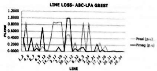
Figure 5.0: Graph Showing ABC_Gbest Line Losses
