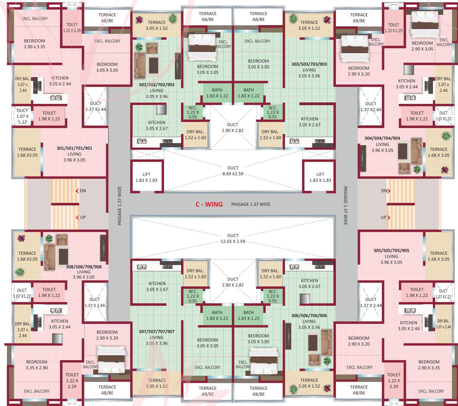
3rd, 5th, 7th & 9th Floor Plan
