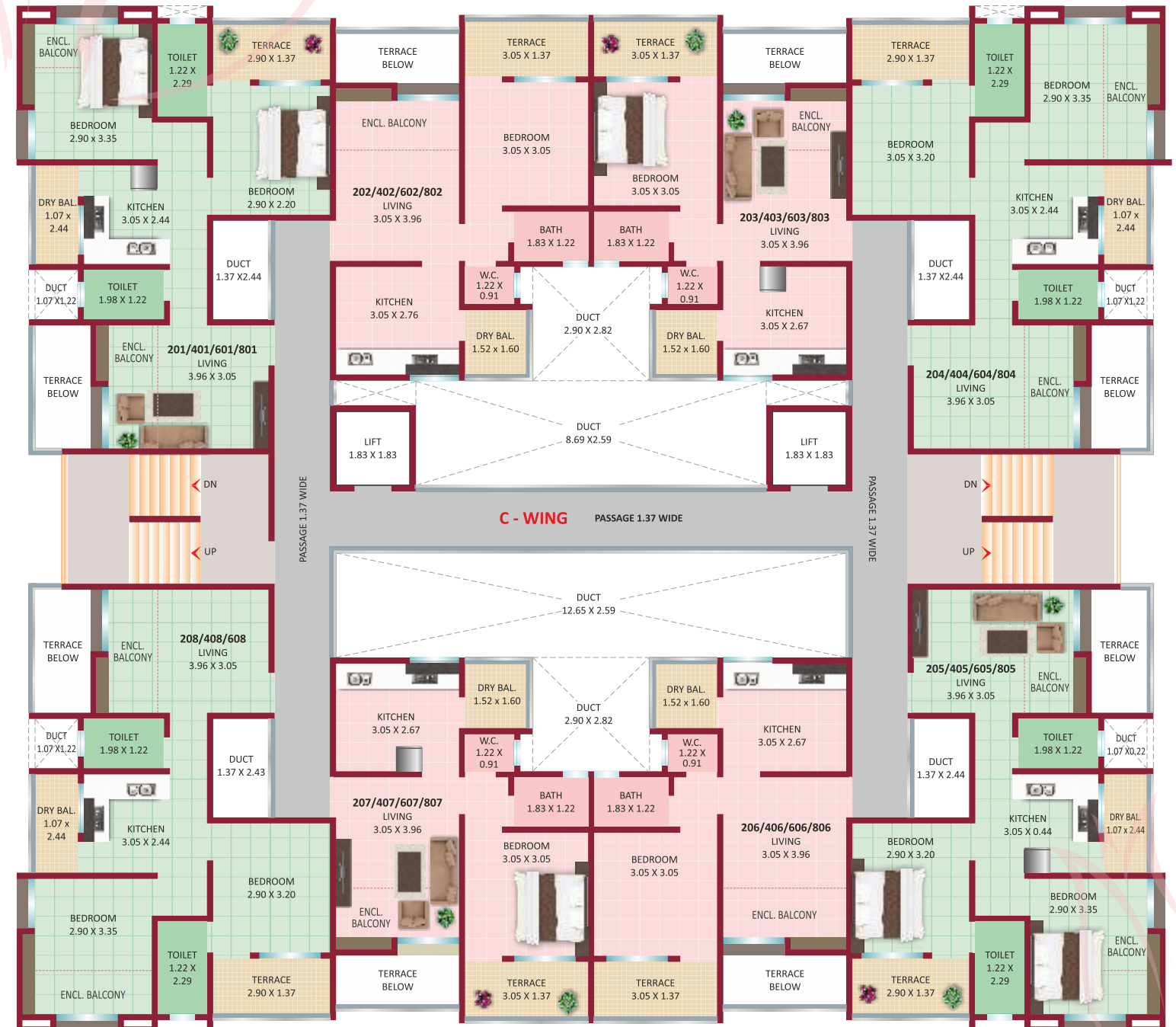
2nd, 4th, 6th & 8th Floor Plan
