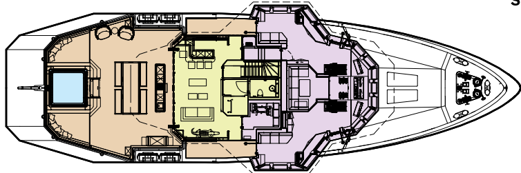
UPPER DECK
