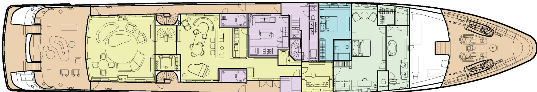
MAIN DECK
