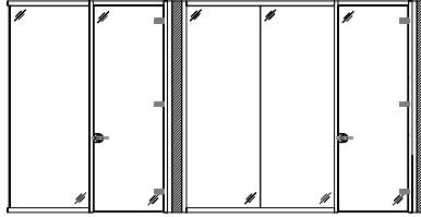
Single Hinged Door: 3/8" Frameless Glass
