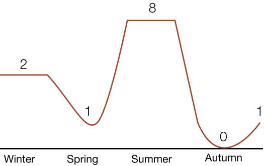
Average Rainfall Days per Month in New Delhi
