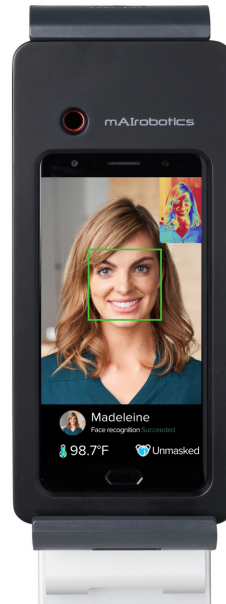
Face Recognition
