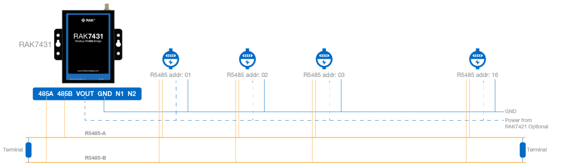
Figure 5: RAK7431 WisNode Bridge Serial ModBus connection diagram
