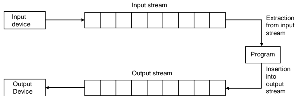
Figure 1.1 Data Streams
