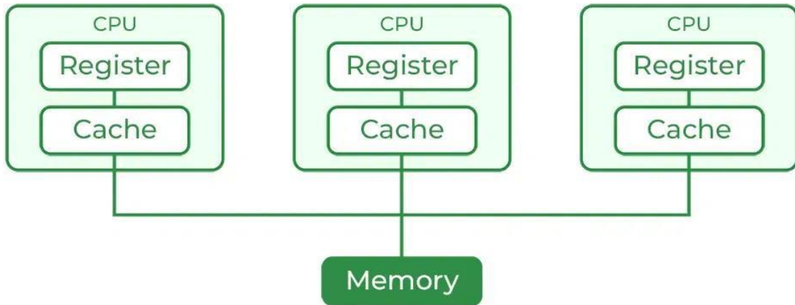
Multiprocessing
