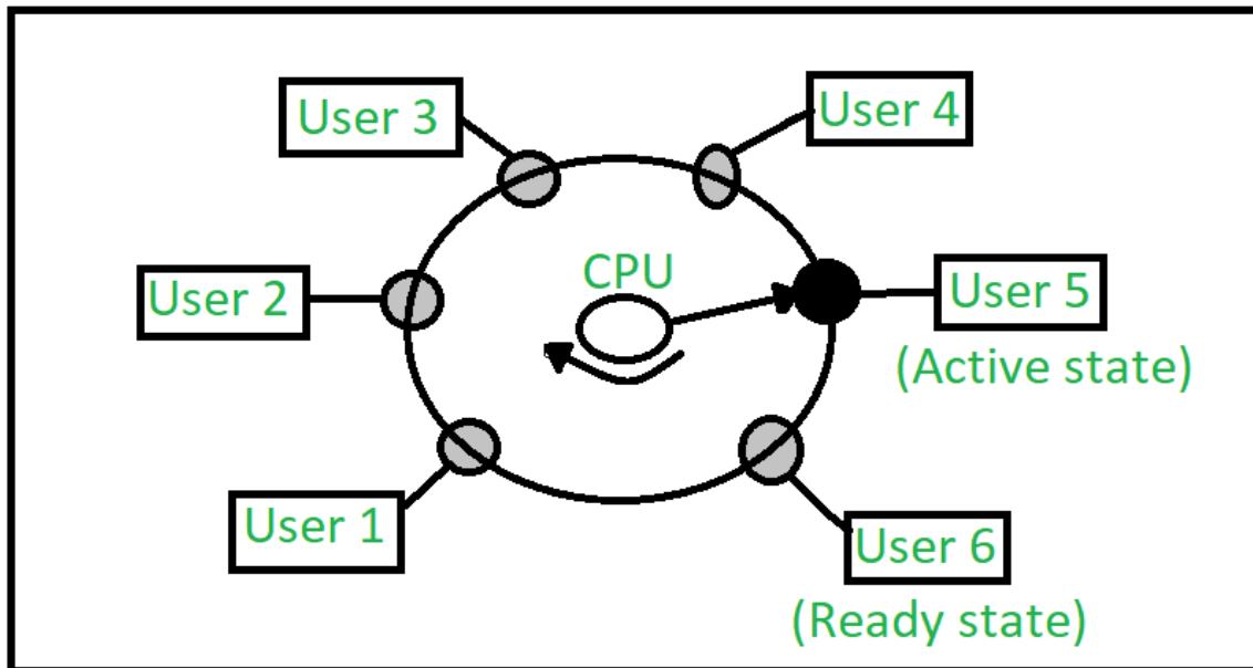
Time-Sharing OS
