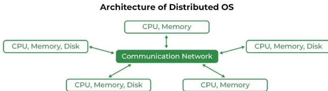
Distributed OS
