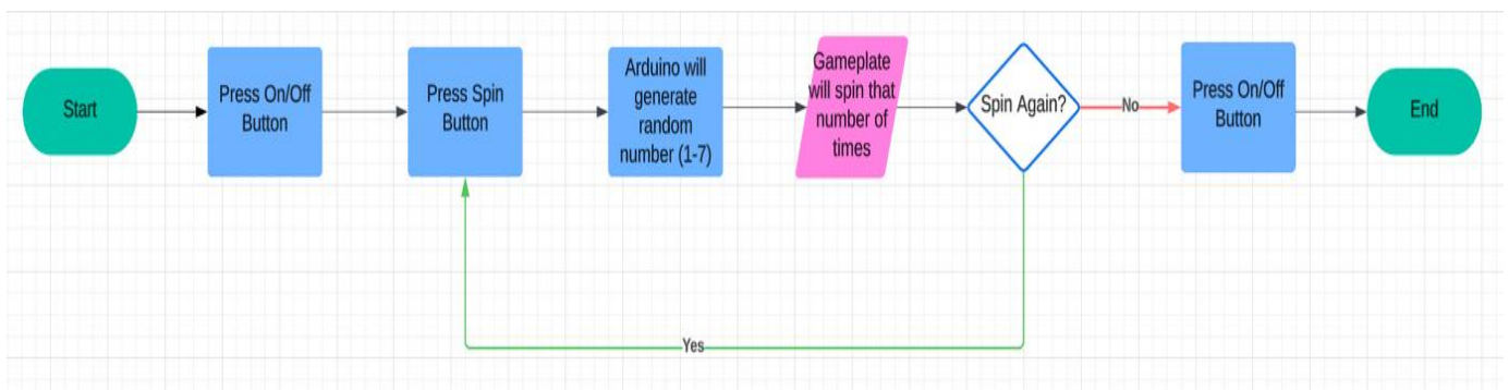
Figure 4: Flowchart of the Algorithm of the Game Spinner System
