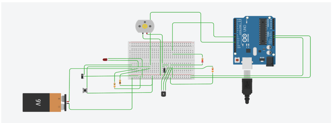
Figure 5: Modelling of the electronic subsystem of the Mechatronic Spinner System
