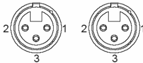
XLR 3p Female-panel Pinout
