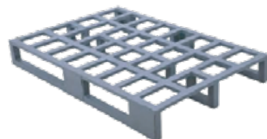
Model Name: Industrial Floor Moving Pallet Model No. SMIP-0001 Model Size: As per Customer Requirements.
