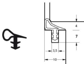
Part number S 485/10 Material TPE Pack. unit 200 m coil
