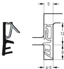
Part number SP 7612 Material TPS Pack. unit 200 m spool
