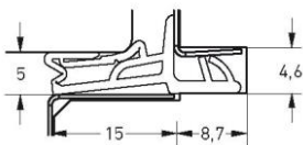
Part number S7312 Material TPE Pack. unit 150 m spool
