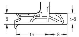
Part number S7322 Material TPS Pack. unit 150 m spool
