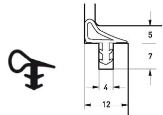
Part number S 485 Material TPE Pack. unit 150 m coil
