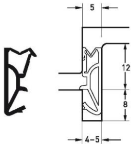
Part number SV 12 Material TPE Pack. unit 200 m spool
