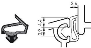
Part number SP 6919a Material TPS Pack. unit 200 m spool
