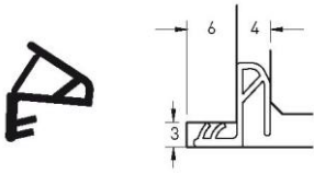
Part number S 7442 Material TPE Pack. unit 250 m spool
