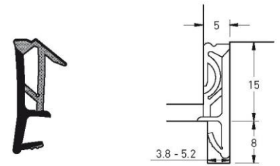
Part number SPV 15 Material TPE Pack. unit 150 m spool
