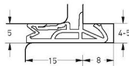
Part number S7672 Material TPE Pack. unit 150 m spool
