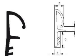
Part number S 7326 Material TPE Pack. unit 160 m coil
