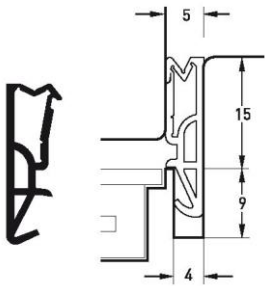
Part number SV 415a Material TPE Pack. unit 150 m spool
