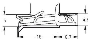
Part number S7346 Material TPE Pack. unit 100 m coil
