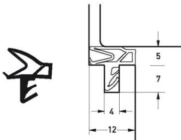
Part number S 6577 Material TPE Pack. unit 200 m spool
