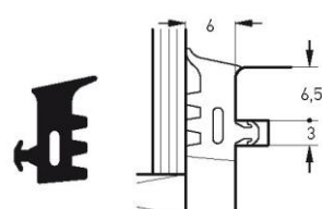
Part number S 7636 Material TPE Pack. unit 200 m spool
