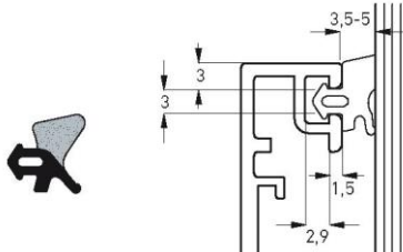
Part number DS 7354 Material silicone Pack. unit 100 m spool
