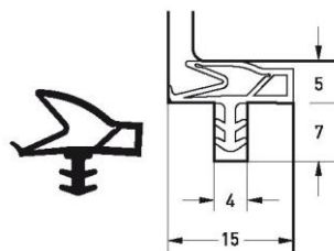
Part number S 6699 Material TPE Pack. unit 150 m spool
