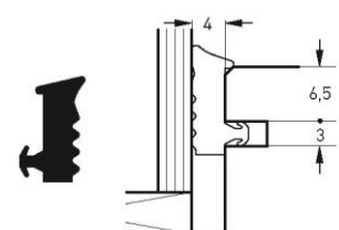
Part number S 7634 Material TPE Pack. unit 200 m spool
