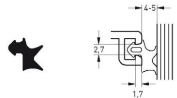
Part number DS 7620 Material silicone Pack. unit 100 m spool
