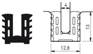
Part number M 7287 Material PVC Pack. unit 100 m spool
