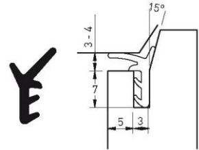
Part number S 3223a Material TPE Pack. unit 300 m spool
