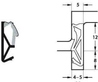
Part number SP 812 Material TPS Pack. unit 200 m spool
