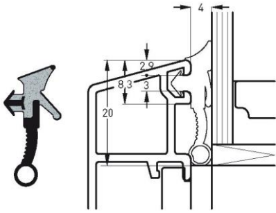
Part number SP 6881 b Material TPS Pack. unit 150 m spool
