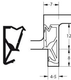
Part number S 6624 Material TPE Pack. unit 150 m spool
