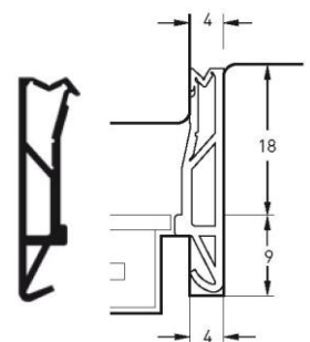
Part number SV 180 Material TPE Pack. unit 150 m spool
