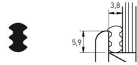
Part number M 7242 Material PVC Pack. unit 400 m spool
