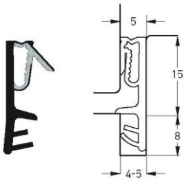
Part number SP 7715 Material TPE Pack. unit 100 m spool
