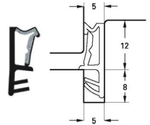
Part number SP 6850 Material TPS Pack. unit 200 m spool
