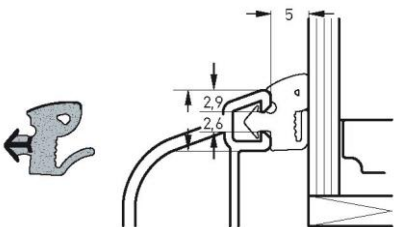
Part number SP 6942 Material TPS Pack. unit 250 m spool
