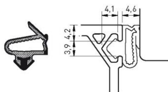
Part number SP 6920a Material TPS Pack. unit 200 m spool
