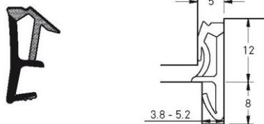
Part number SPV 12 Material TPE Pack. unit 180 m spool
