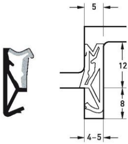
Part number SP 125 Material TPS Pack. unit 200 m spool
