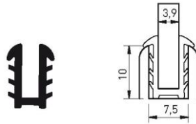
Part number M 7582 Material PVC Pack. unit 250 m spool
