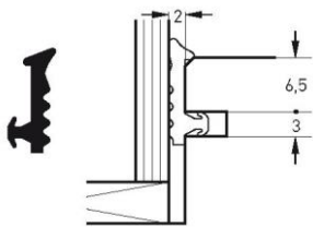
Part number S 7632 Material TPE Pack. unit 400 m spool
