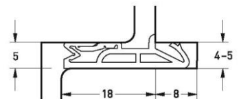
Part number SV185 Material TPE Pack. unit 150 m spool
