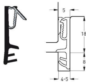
Part number SP 7718 Material TPE Pack. unit 125 m spool
