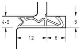
Part number S6512a Material TPE Pack. unit 180 m spool
