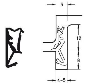
Part number SV 125 Material TPE Pack. unit 200 m spool
