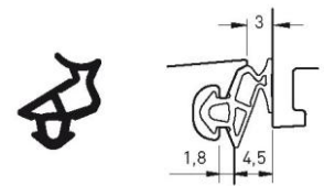
Part number S 7338 Material TPS Pack. unit 200 m spool
