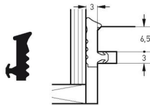
Part number S 7633 Material TPE Pack. unit 400 m spool
