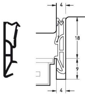
Part number SV 418 Material TPE Pack. unit 150 m spool
