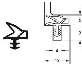
Part number DS 6577 Material TPE Pack. unit 50 m coil
