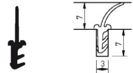
Part number S 6782 Material TPE Pack. unit 300 m spool
