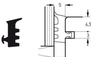
Part number S 7635 Material TPE Pack. unit 200 m spool
