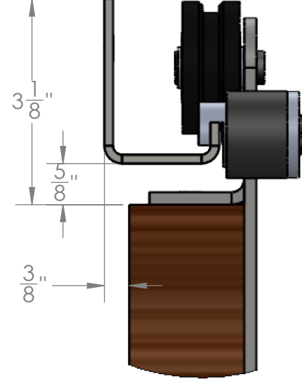
DETAIL A SCALE 1 : 2
