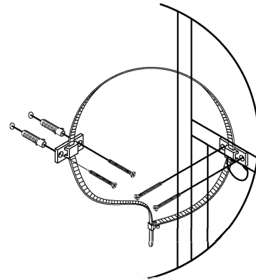
Enlarged View of Section C
