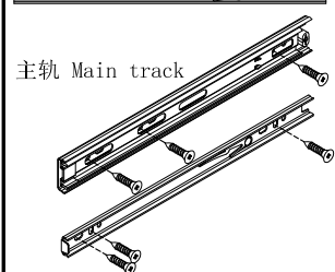
三节滚珠导轨-12" Three-section rail
