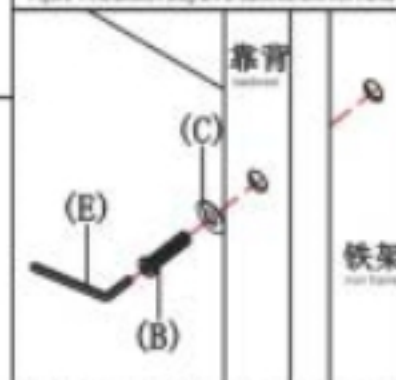
图2:前挡板和铁架安装示意图(1) Figure 2: installation diagram of front baffle and iron frame (1)
