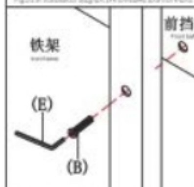
图3:前挡板和铁架安装示意图(2) Figure 3: installation diagram of front baffle and iron frame (2)
