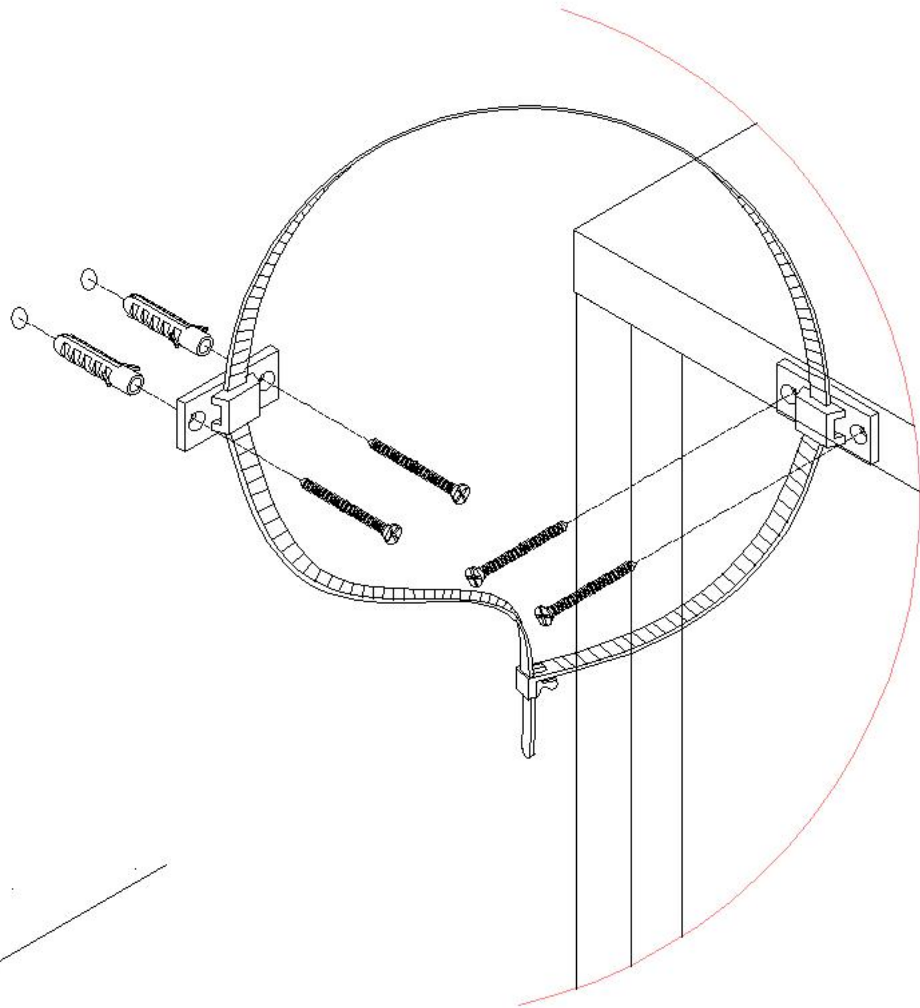
I处放大图 Enlarged view at I
