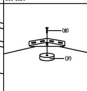
图3: 床尾脚安装示意图 Figure 3: Installation diagram of bed foot
