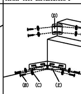
图2: 角码安装示意图1 Figure 2: Schematic diagram of corner code installation 1
