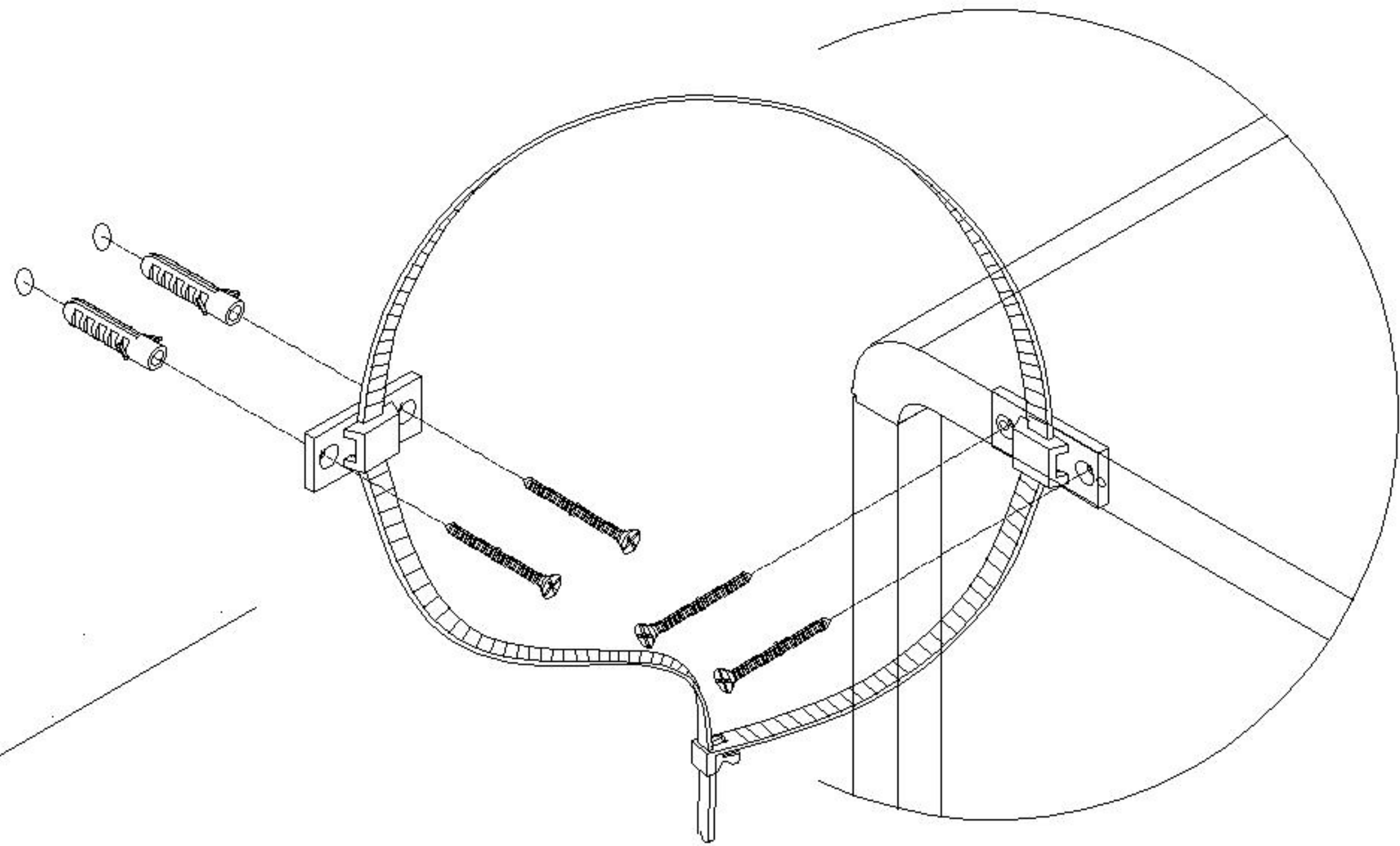
J处放大图 Enlarged view at J
