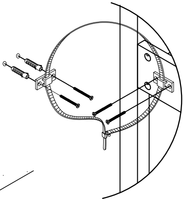
Y处放大图 Enlarged view at Y
