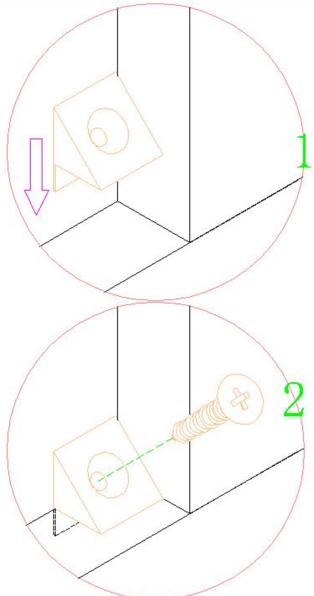
背板扣 Back Plate Buckle-White
