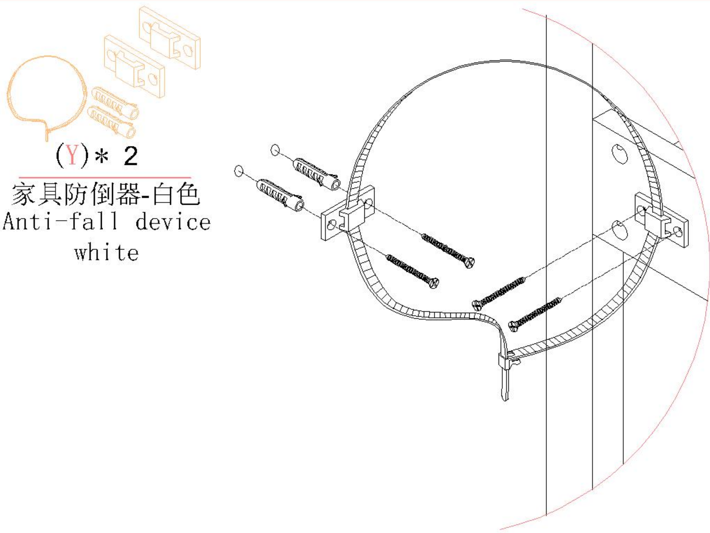
Y处放大图 Enlarged view at Y
