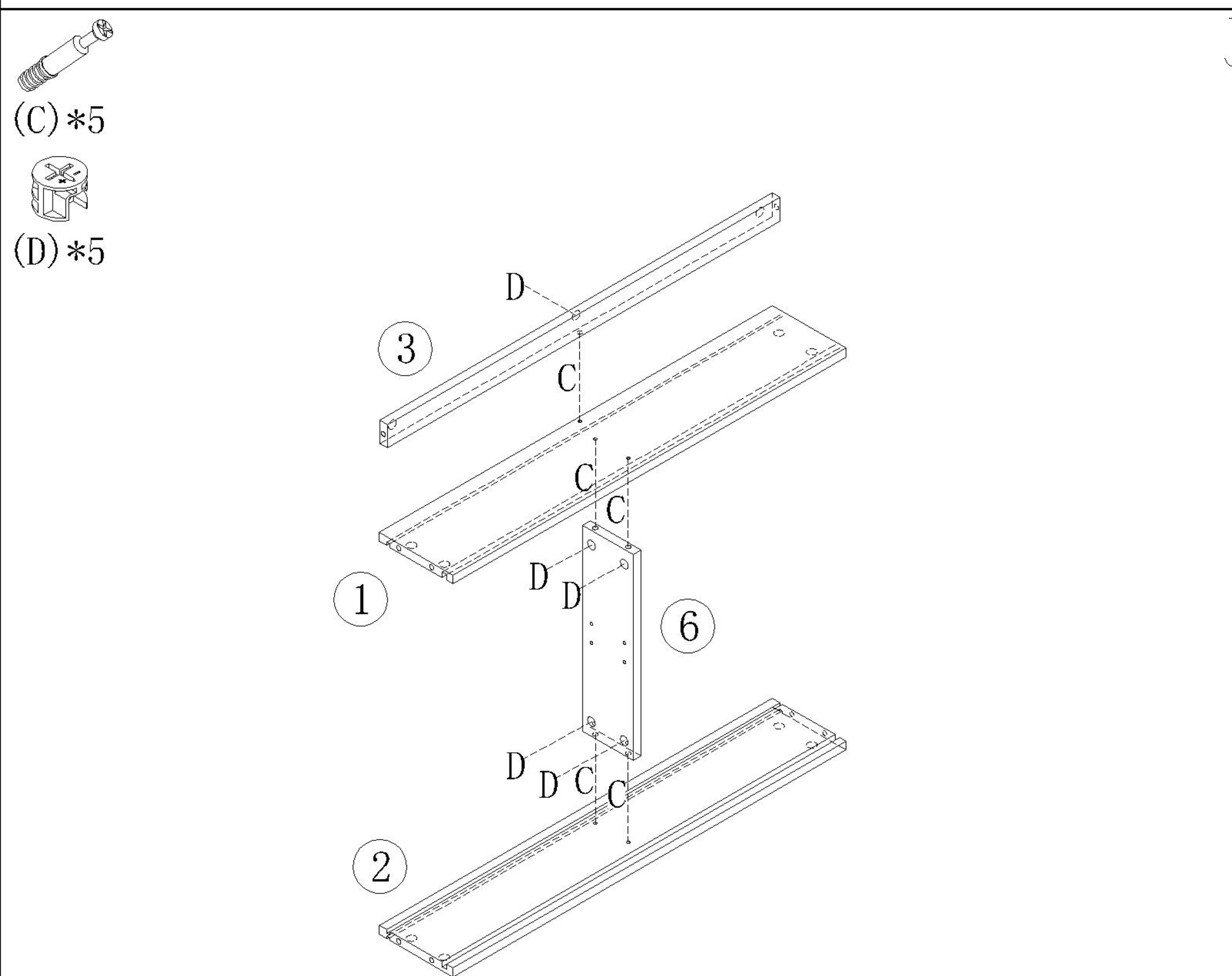
副轨 Sub track
